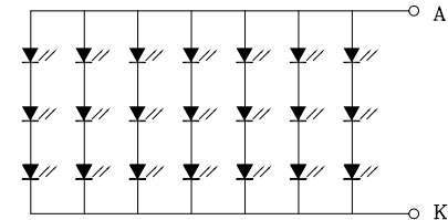
LED CIRCUIT DIAGRAM 9.6V@180mA
