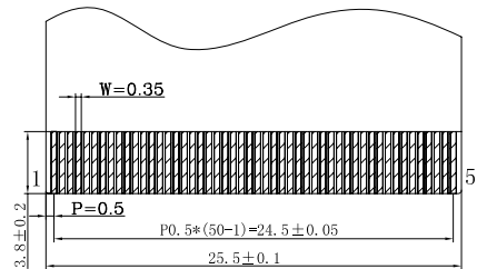
DETAIL A 5:1
